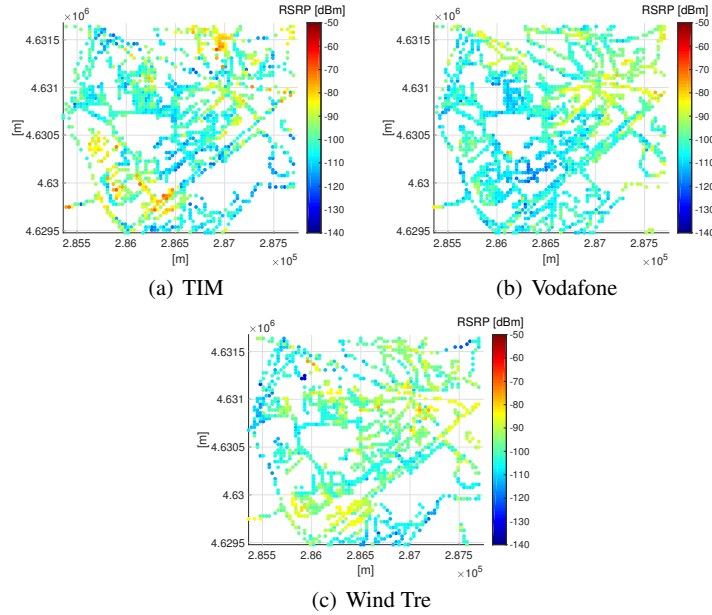
Fig. 3 RSRP metric (TMC case-study) [4].
