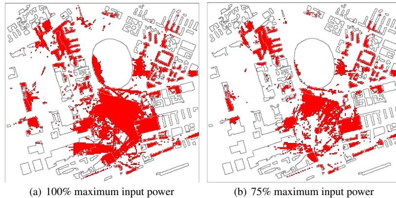
Fig. 2 Impact of the maximum input power (Fuorigrotta case-study) [4].
